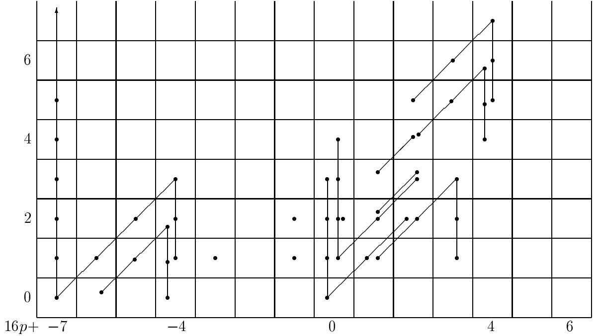
Diagram 2.2. Adams spectral sequence of \Sigma P_{16p-8}
