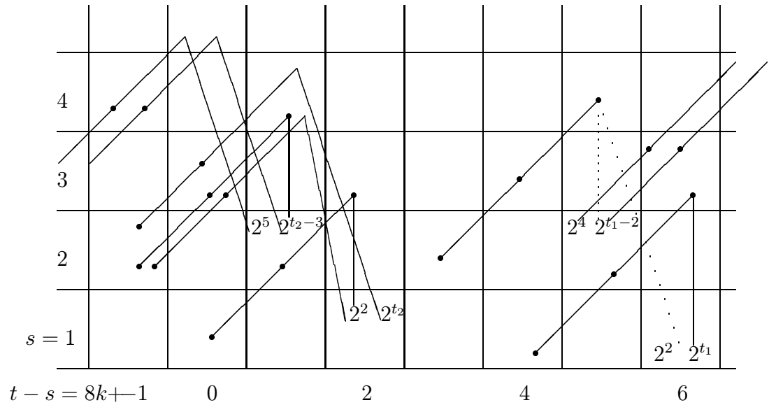
Diagram 5.11. The BTSS of E_7
