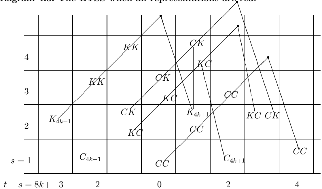
Diagram 4.3. The BTSS when all representations are real
