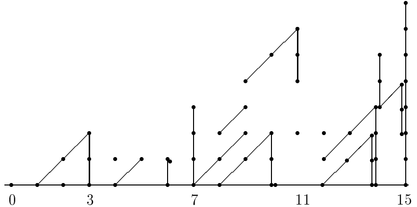
Diagram 2.2. E_2(\mathrm{tmf}_*(P_{-3} \wedge P_3)) , * \leq 15
