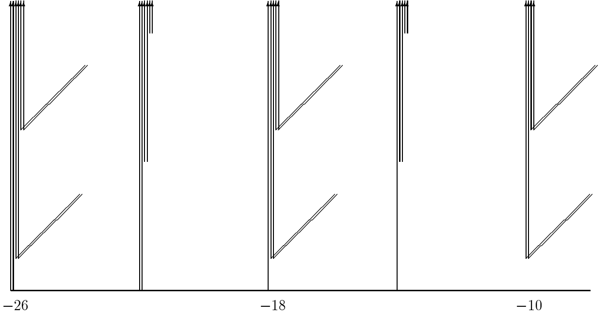
Diagram 3.18. Illustration of Proposition 3.15
