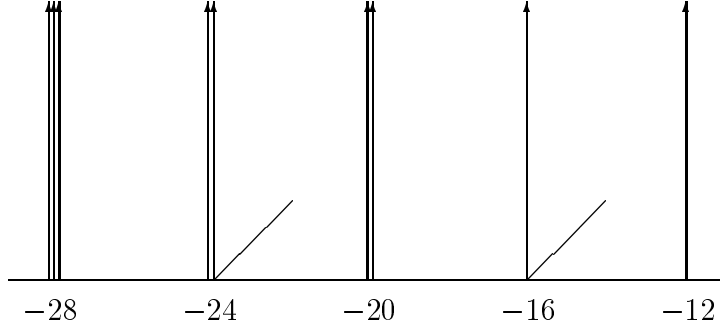
Diagram 5.11. Structure on two types of generators
