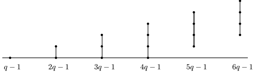
Figure 2. ASS for \ell_*(B^{4q}) for t - s < 6q
