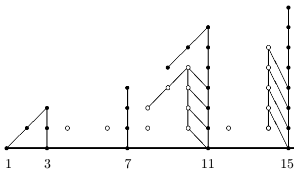
Figure 10. J_*(P^{2m}) in * \leq 15 , provided m \geq 8
