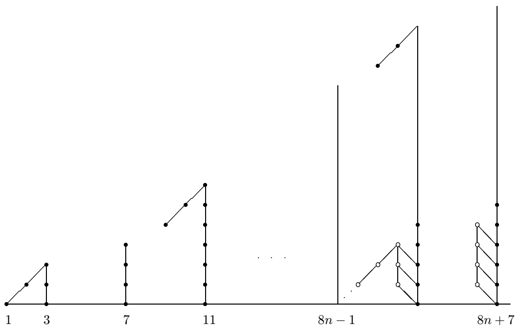
Figure 9. bo_*(P^{8n}) , from bo_*(P) and bo_*(P_{8n+1})
