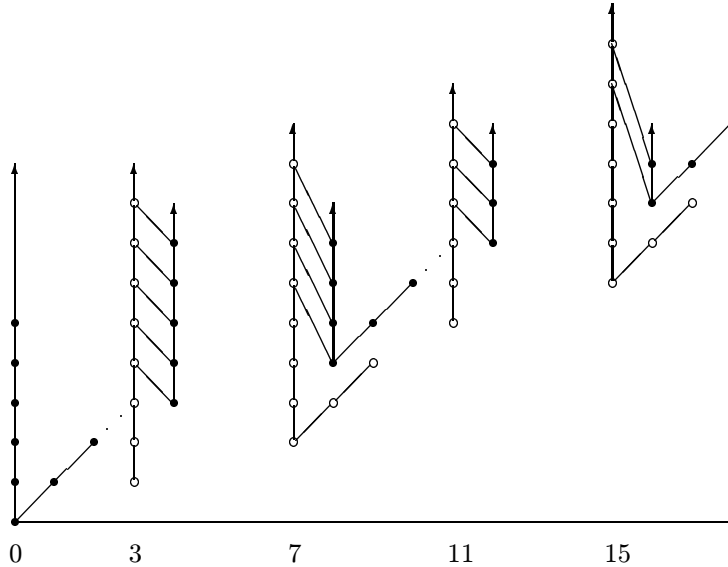
Figure 5. 2-primary \pi_i(J) , i \leq 18
