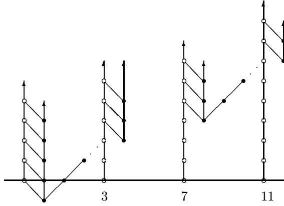
Figure 6. Ext_{A_1}(H^*P) , from Ext_{A_1}(H^*S^0) and Ext_{A_1}(H^*R) , t - s < 15
