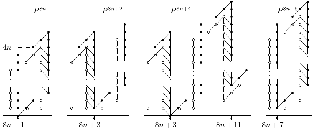
Figure 11. J_*(P^{2m}) where it starts to ascend
