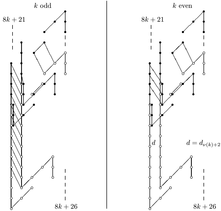
Figure 17. Final chart for v_1^{-1}\pi_*(F_4/G_2)
