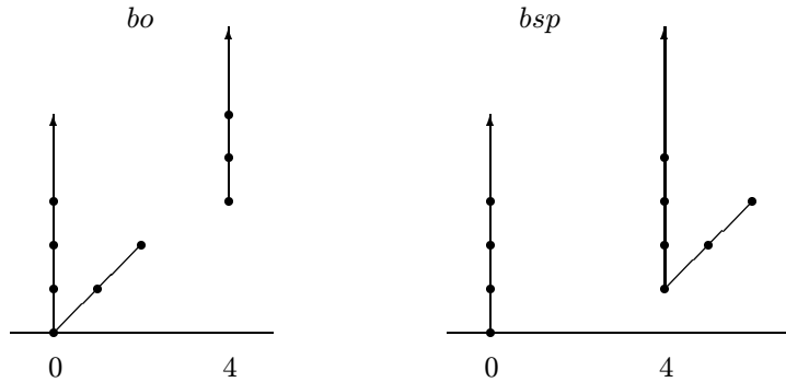
Figure 4. Part of ASS for bo and bsp
