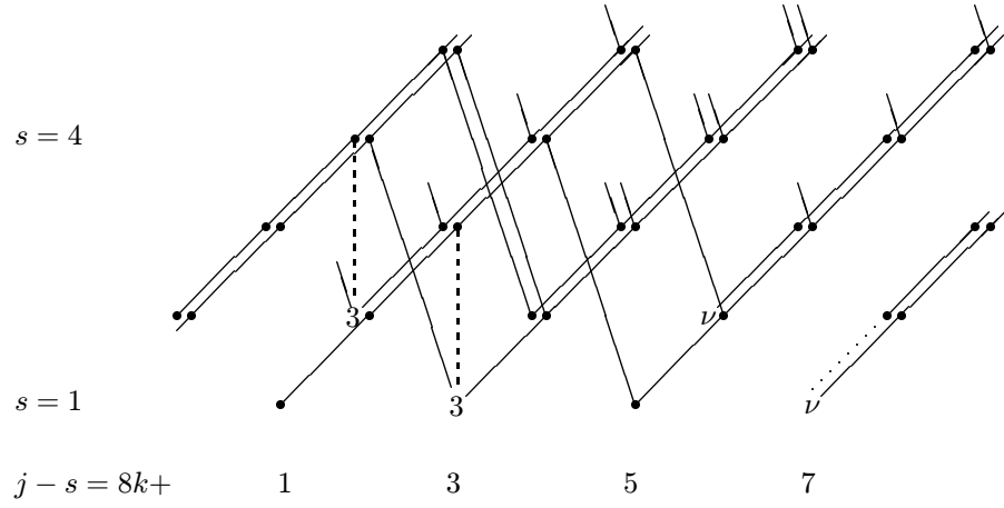
Figure 13. v_1^{-1}E_2^{s,2n+1+j}(S^{2n+1}) , n \equiv 0, 3 \pmod 4 , p = 2
