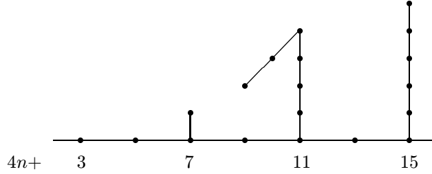
Figure 8. bsp_*(P_{4n+3}), * \leq 15
