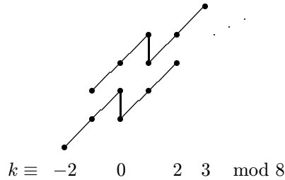
Figure 12. \mathit{dirlim}_i [\in^{k+8i} M, J]
