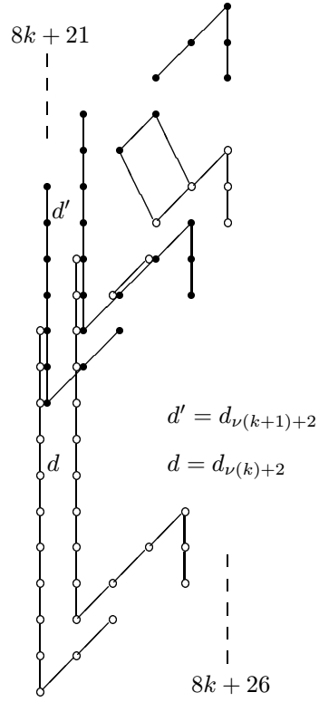
Figure 15. Initial chart for v_1^{-1}\pi_*(F_4/G_2)
